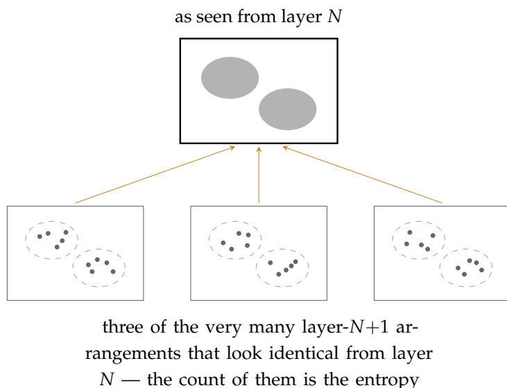
Figure 7.8.: Entropy, layer-indexed. Above: a region as layer N sees it — two bodies, and that is all layer N can say. Below: three of the very many layer- N+1 arrangements that present exactly this appearance. The number of such arrangements — how many ways the crowd below can be while looking the same from above — is the region’s entropy at layer N . The line between tracked and ignored is not chosen by an observer; it is drawn by the world, once per layer — and the exactness of the crowd’s species (the fourth wound) is what makes the count well defined.
