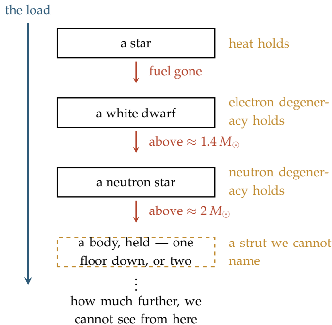
Figure 7.9.: The ladder under load. Each rung is the same event at a finer scale: a structure’s resistance is exceeded, its constituents are crushed into a smaller arrangement, and that arrangement’s own stiffness takes the weight. The first three rungs are observed — our sun will make the second, and we have photographed the third. The standard picture has no fourth rung and puts a singularity there instead: everything, in no volume at all, which is a floor by another name. The tower’s fourth rung is an ordinary thing in extraordinary circumstances — a body, held up by the layer below.
